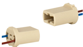
141211 Lamphouder G9 6A 250V T250°C 250mm
