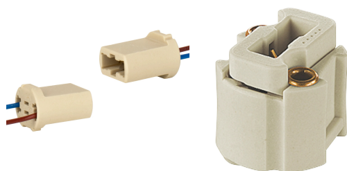
141211 Lamphouder G9 6A 250V T250°C 250mm
