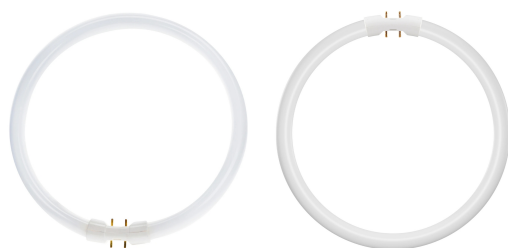
146255 TL5 Circular 2GX13 22W 1320lm 840 146564 LED Circular T5 2GX13 11.6W (22W) 33V 1700lm 840
