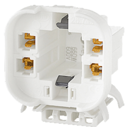
140261 BJB 26.745.1801.50 GX24q (without key) Douille Snap in
