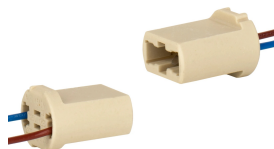
141211 Douille G9 6A 250V T250°C 250mm
